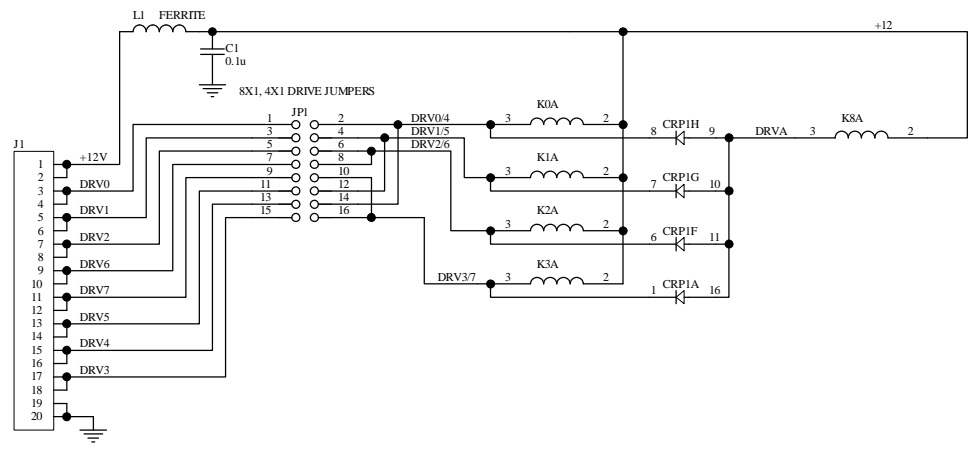
J1 - RELAY DRIVE CONNECTION
